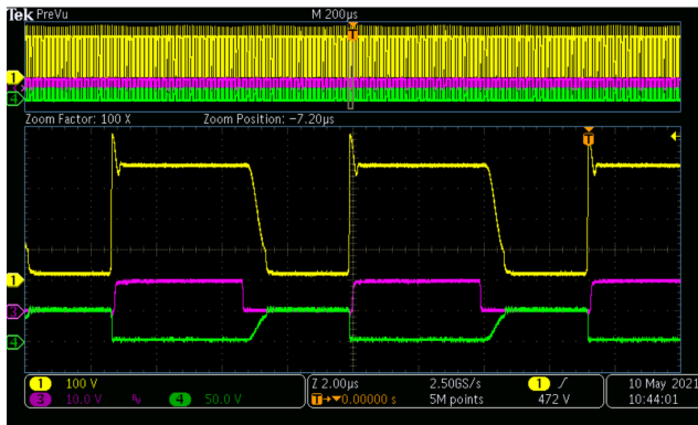
Figure 42. 90 Vac (CH1: Vds_sec, CH2: Vdrv)
