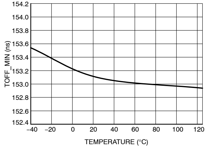
Figure 19. T_{\text{OFF\_MIN}} vs. T at V_{\text{HVBias}} = 48\text{ V}
