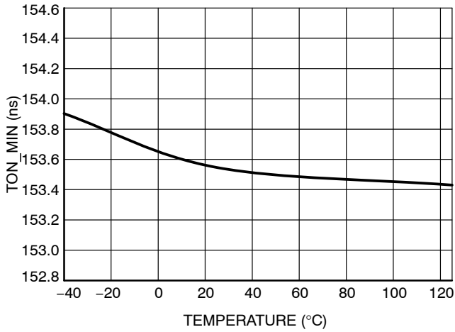
Figure 18. T_{\text{ON\_MIN}} vs. T at V_{\text{HVBias}} = 48\text{ V}
