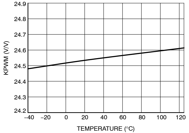
Figure 17. PWM Modulator Gain, V_{\text{IN}} / \Delta V_{\text{RAMP}} vs. T at V_{\text{HVBias}} = 48\text{ V}
