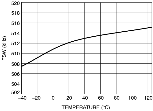
Figure 16. Switching Frequency vs. T at V_{\text{HVBias}} = 48\text{ V} and RT shorted to GND
