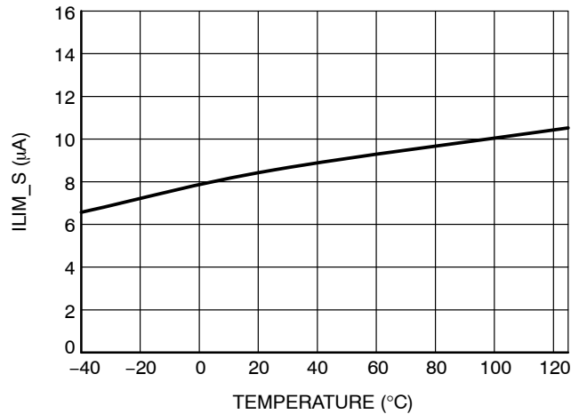
Figure 20. 8.5 \mu\text{A} Current Source for Current Limit Purpose vs. T at V_{\text{HVBias}} = 48\text{ V}
