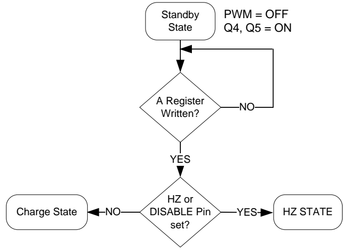
Figure 36. Standby State
