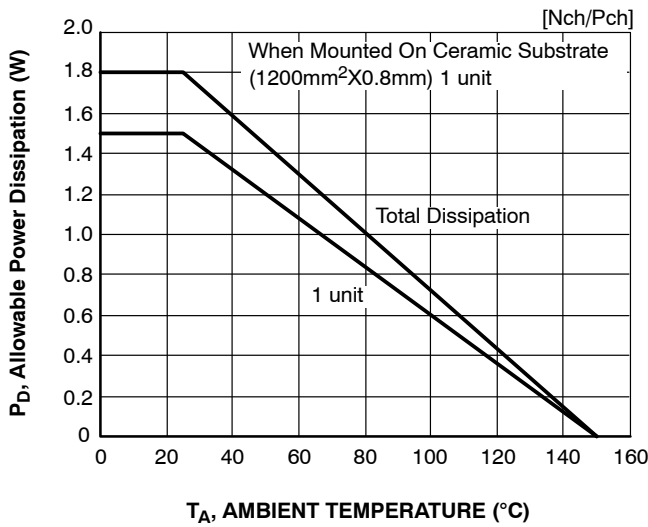
Figure 22. P_D - T_A
