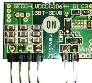
Figure 1. Board Layout
