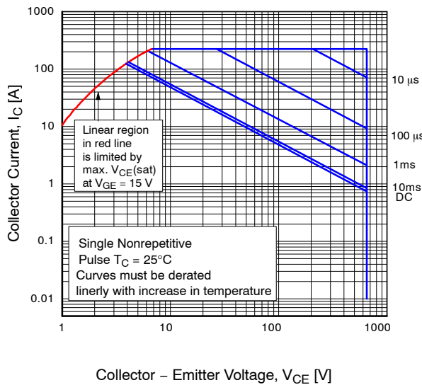
Figure 11. FBSOA Characteristics
