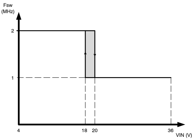
Figure 25. NCV890204 Switching Frequency Reduction at High Input Voltage
