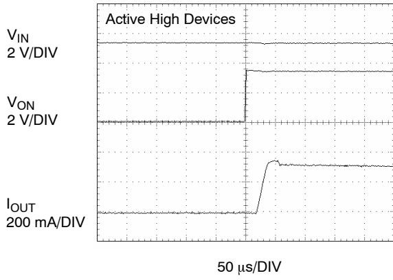
Figure 22. Current Limit Response Time (Output Shorted to GND by 10 Ω, moderate short.)
