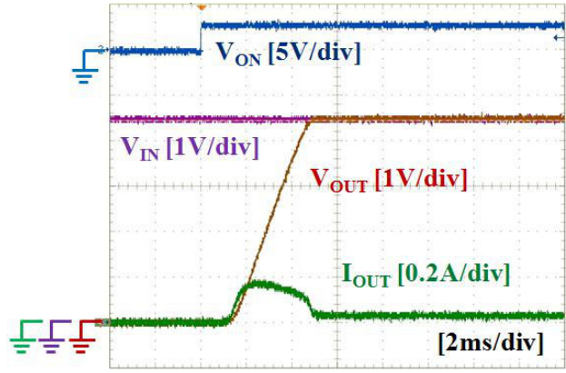
Figure 23. Turn-On Response (V_{IN} = 4.5 \text{ V}, C_{IN} = 10 \mu\text{F}, C_{OUT} = 100 \mu\text{F}, R_L = 150 \Omega)
