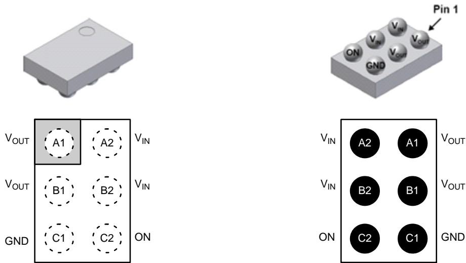
Figure 3. Top View
